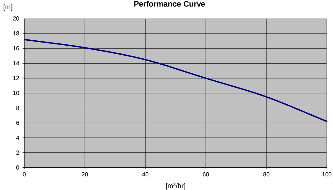
Performance Curve
