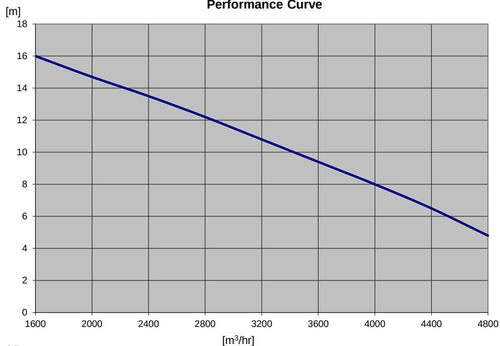
Performance Curve
