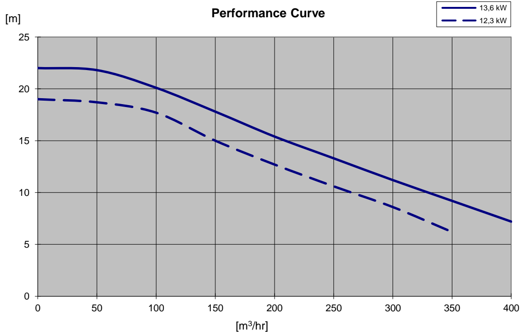
dry installation
