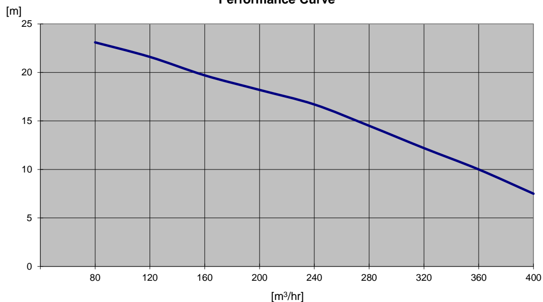
Performance Curve
