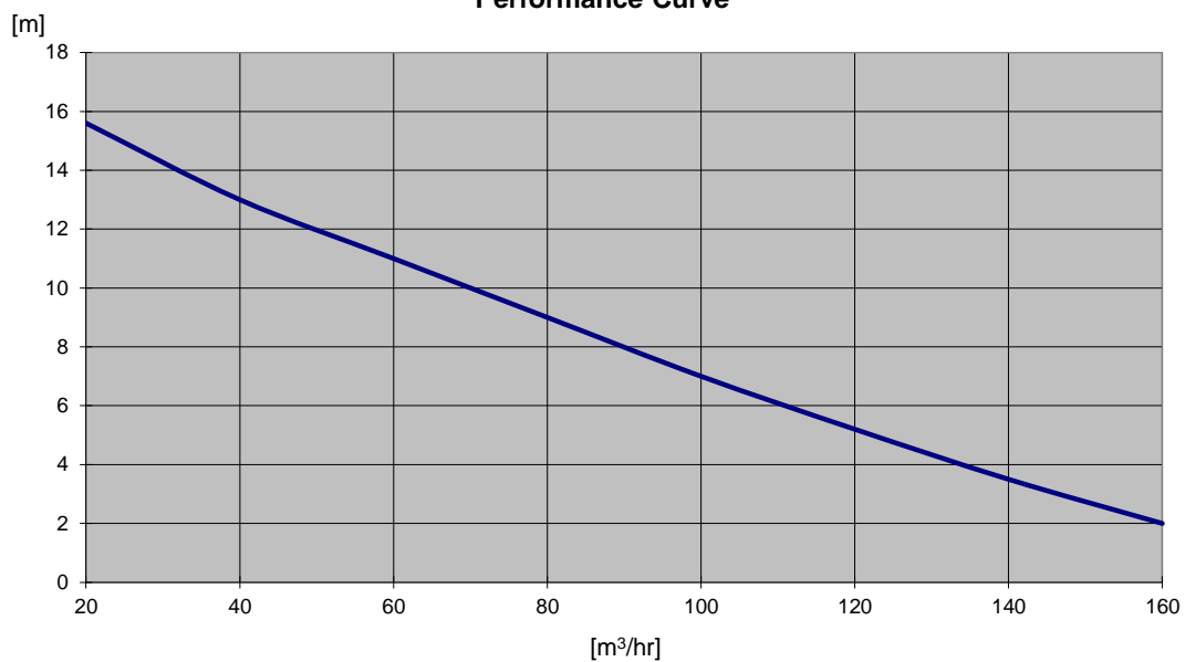
Performance Curve
