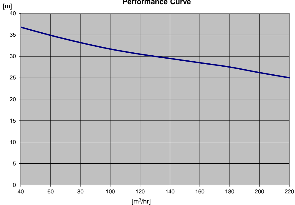
Performance Curve
