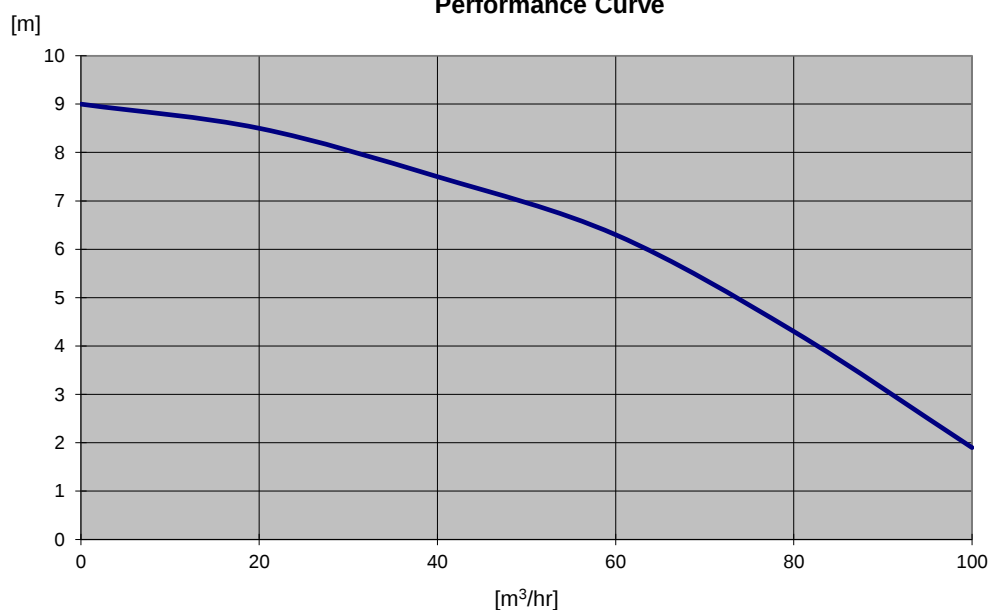
Performance Curve
