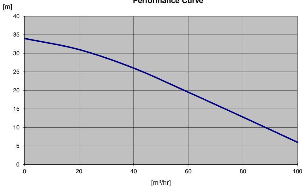
Performance Curve
