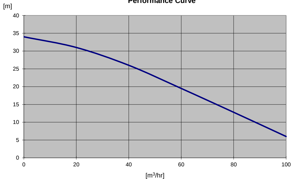
Performance Curve
