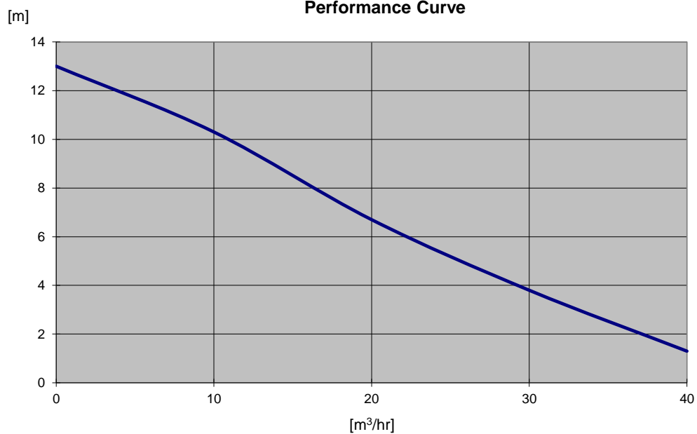
Performance Curve
