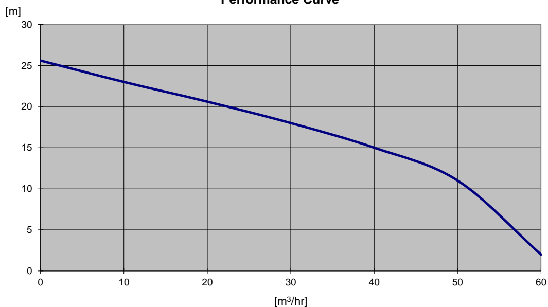
Performance Curve
