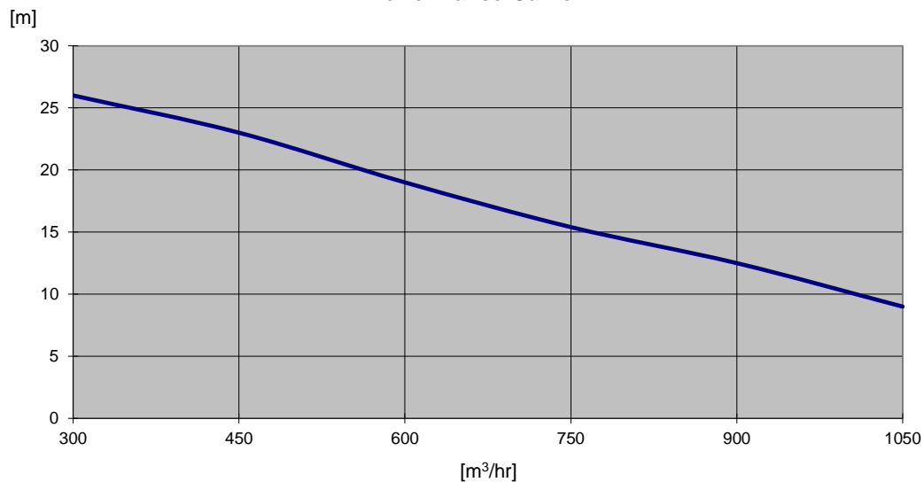
Performance Curve
