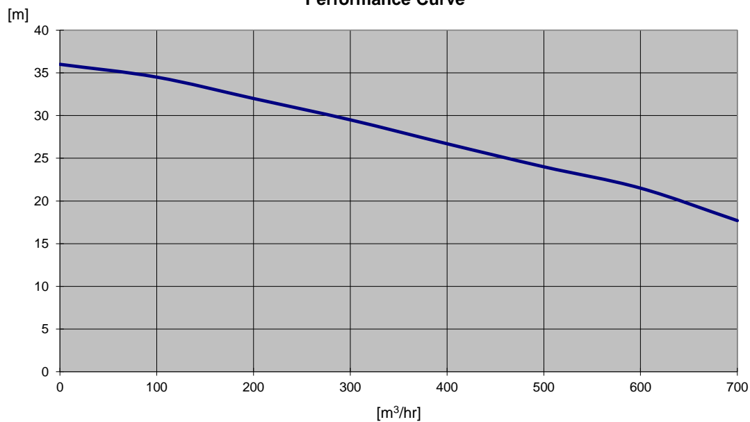
Performance Curve
