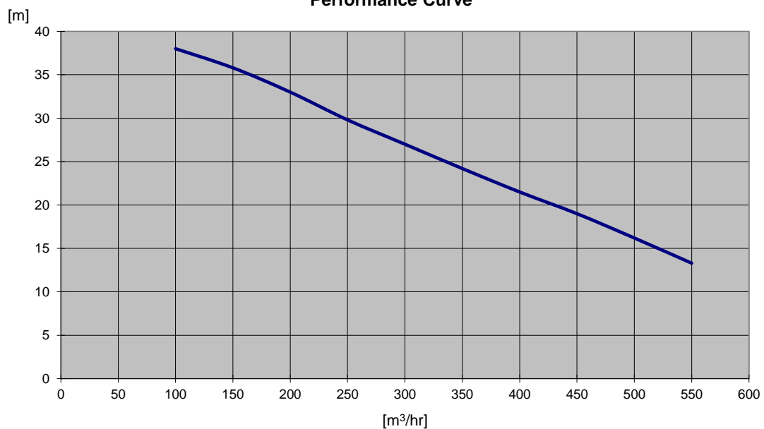
Performance Curve
