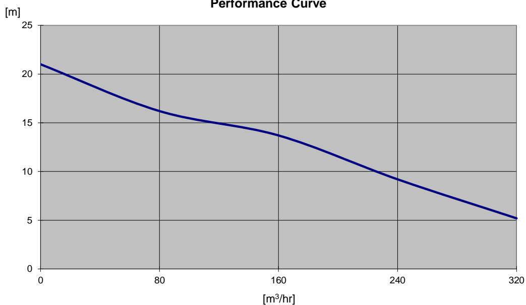
Performance Curve
