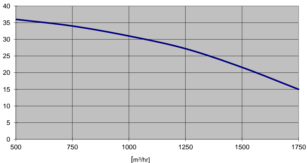
Performance Curve
