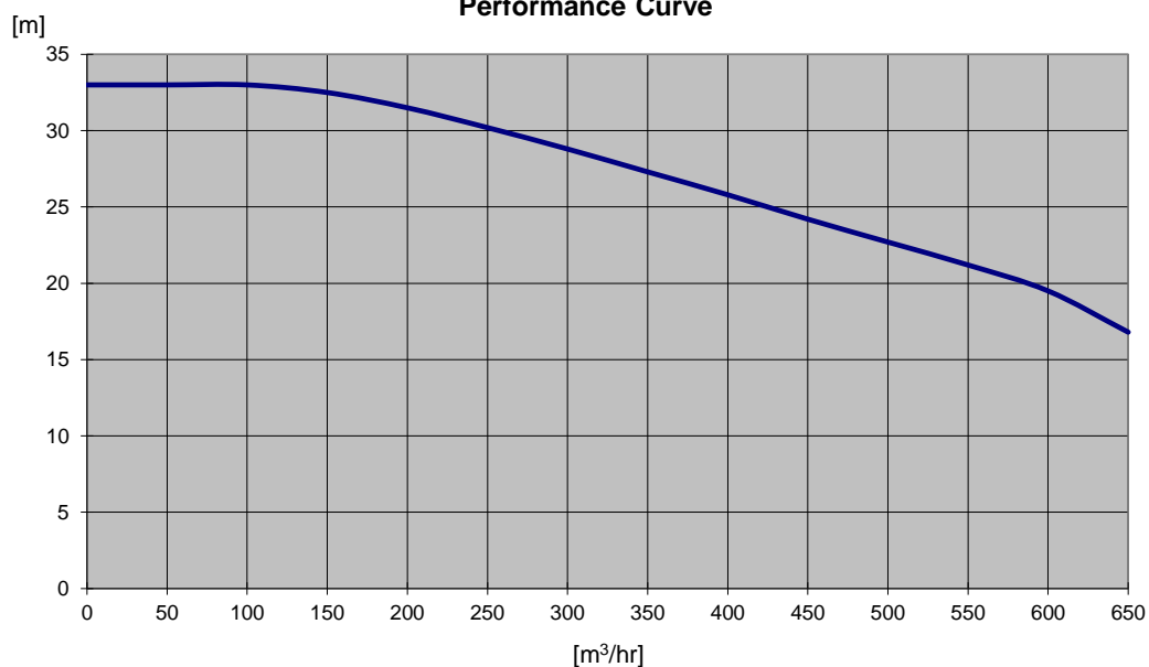
Performance Curve
