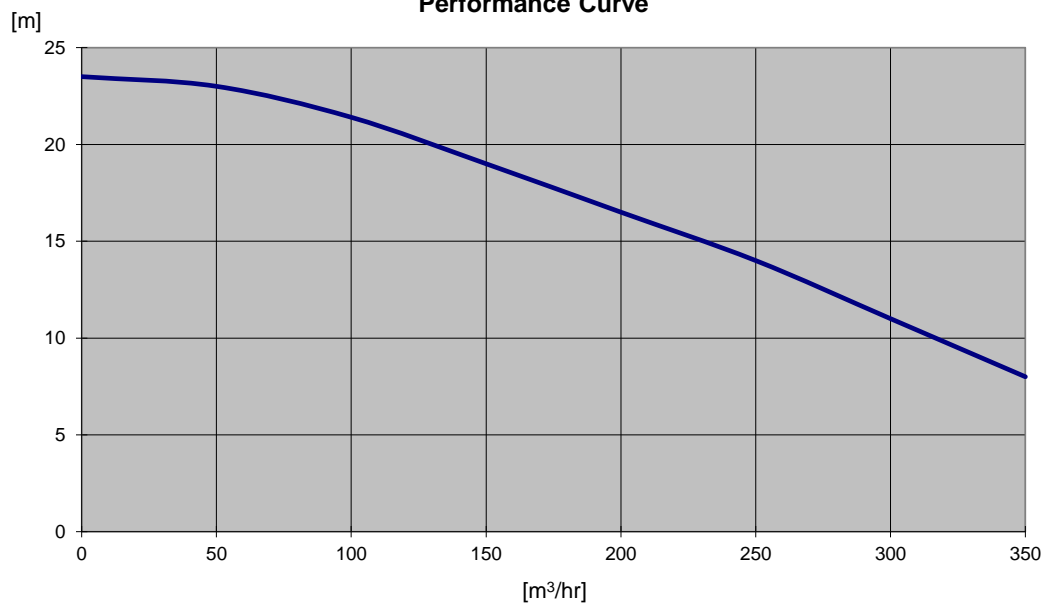
Performance Curve
