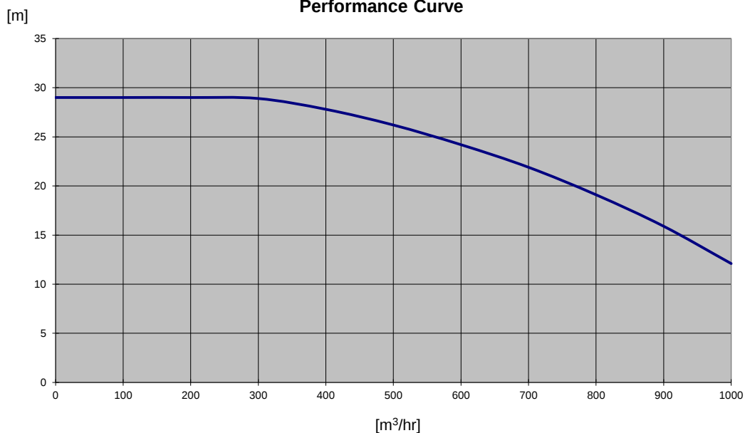
Performance Curve
