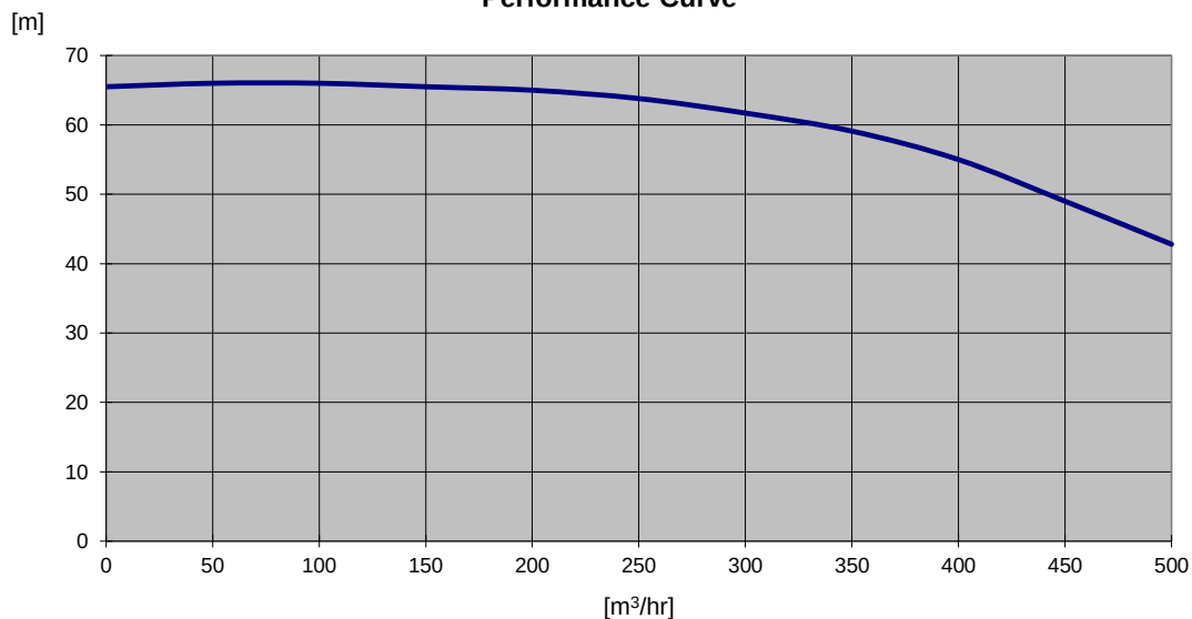
Performance Curve
