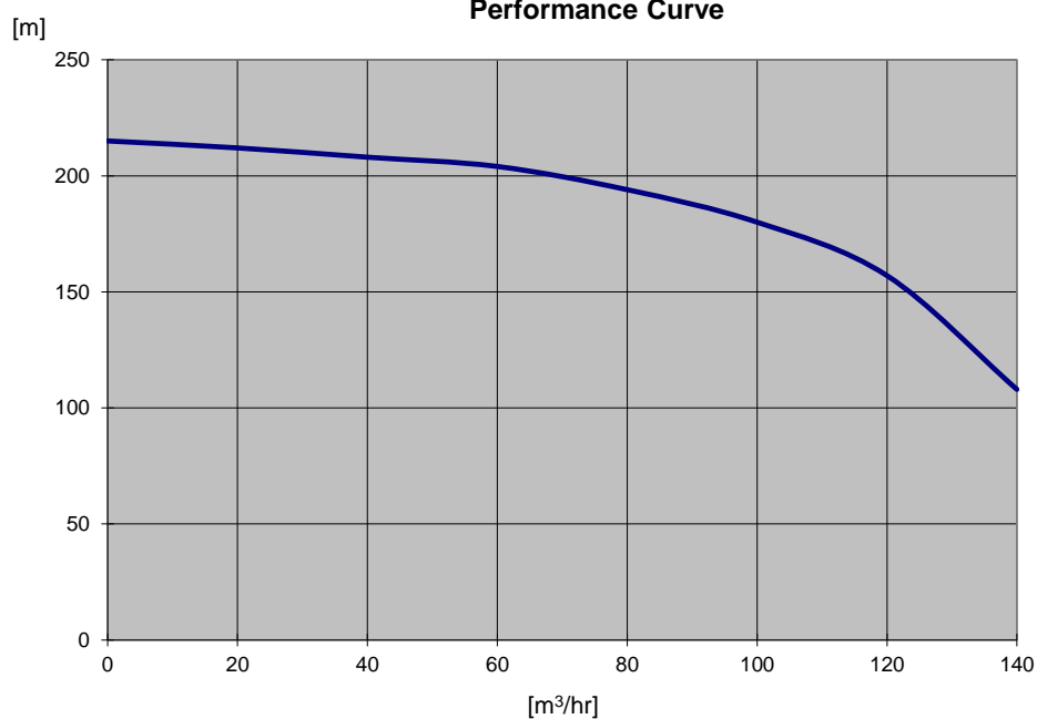
Performance Curve
