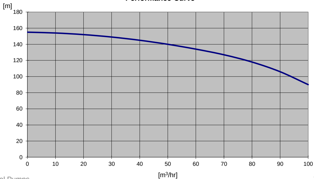
Performance Curve
