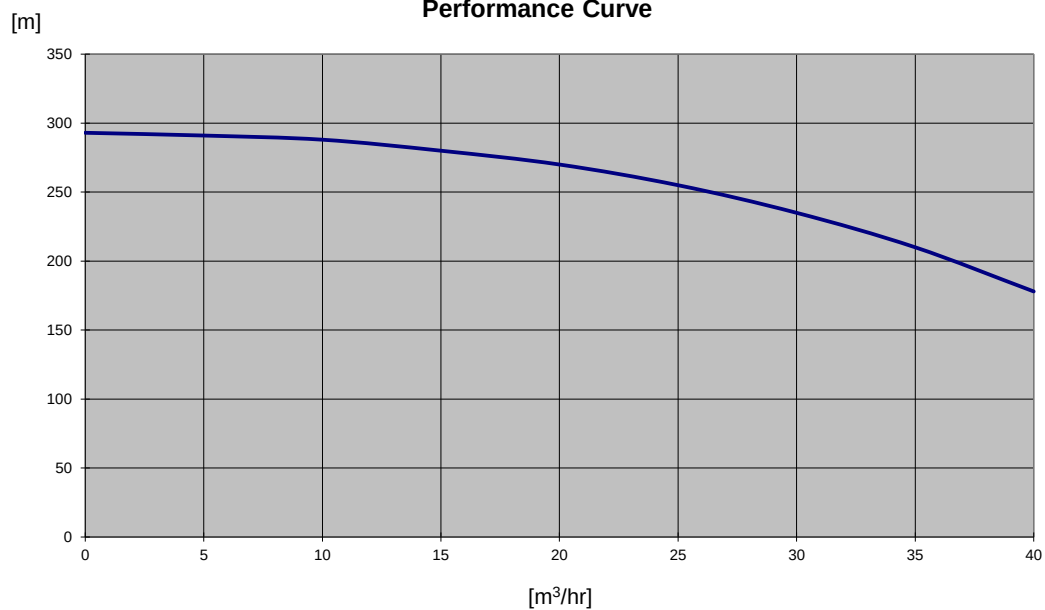
Performance Curve
